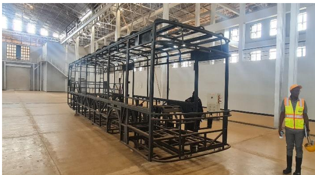
Left: The localized Kayoola EVS Frame at the KMC vehicle plant in Jinja. Right: Fabrication of the 3-in-1 Trike prototype at KMC office in Ntinda
